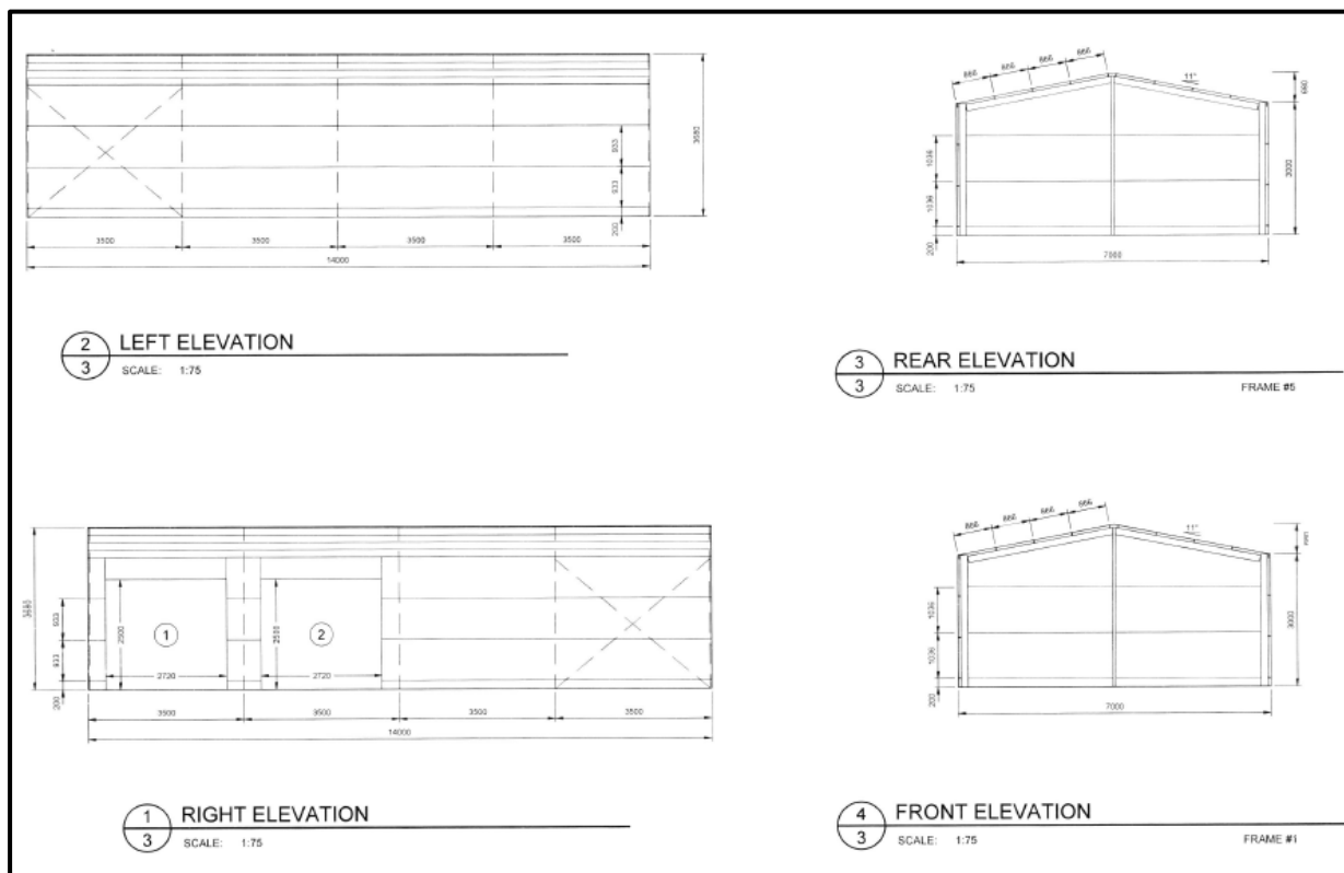
Figure 3 – Elevations Plan
